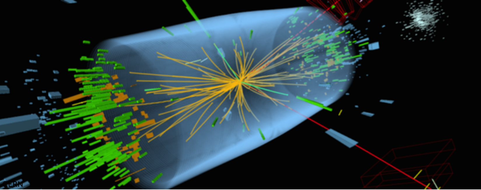
Computer-generated rendering of a particle collision using data from the LHC's detectors, which take snapshots of particle traces.
